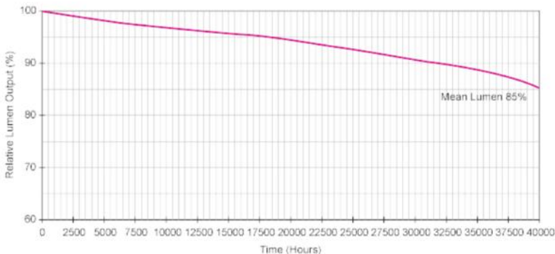
Lumen Maintenance of LED with a Lamp Life of 40000 hours
